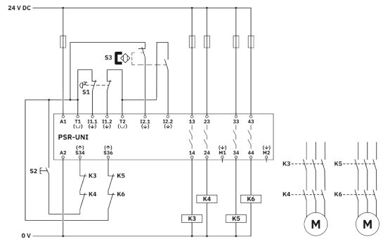
Örnek: PSR-UNI-L-2X2NO-2DO-24DC-PI
